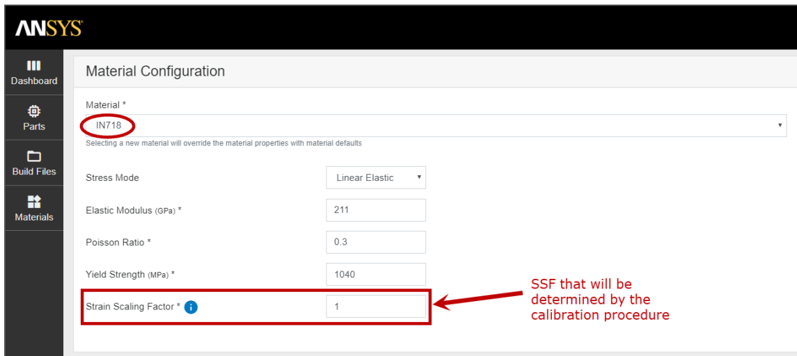
Figure 1: Additive Print application - SSF is required for Assumed Strain simulation type
