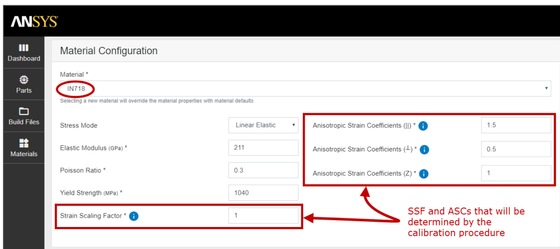
Figure 2: SSF and ASCs are required for Scan Pattern and Thermal Strain simulation types
